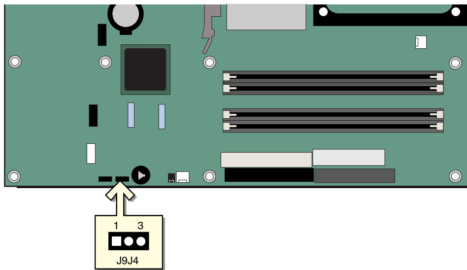
Figure 16. Location of the BIOS Configuration Jumper Block
